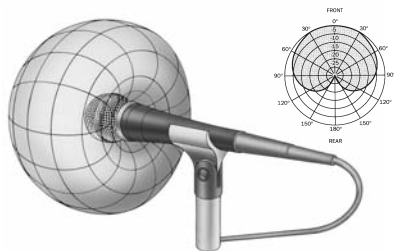
Cardioid (Unidirectional) Microphone
