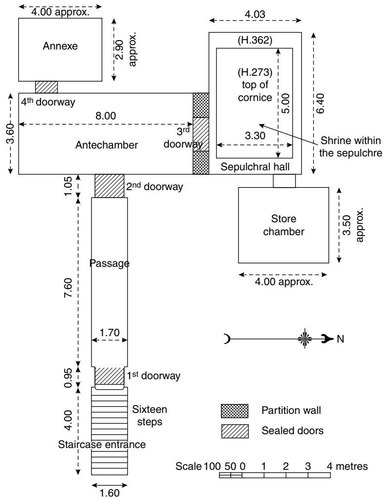
SKETCH-PLAN OF THE TOMB
